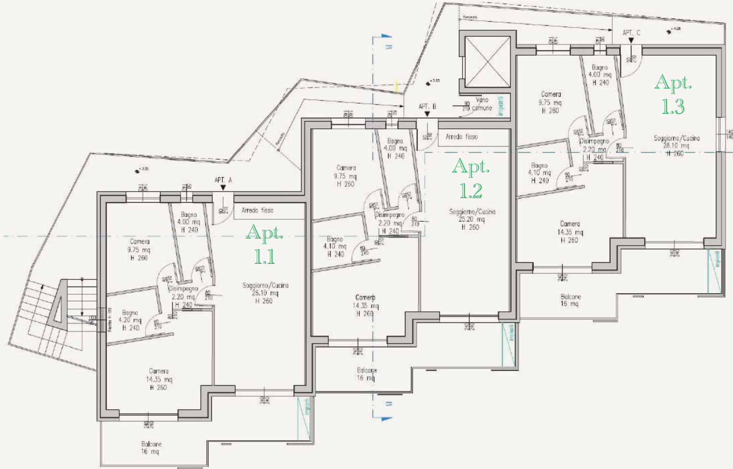
FIRST FLOOR
